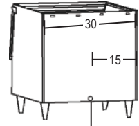
3/4" FPT Drain
